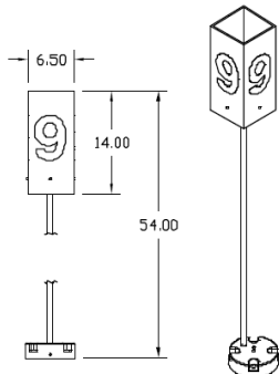
LW000001 LANE LIGHT WHITE
