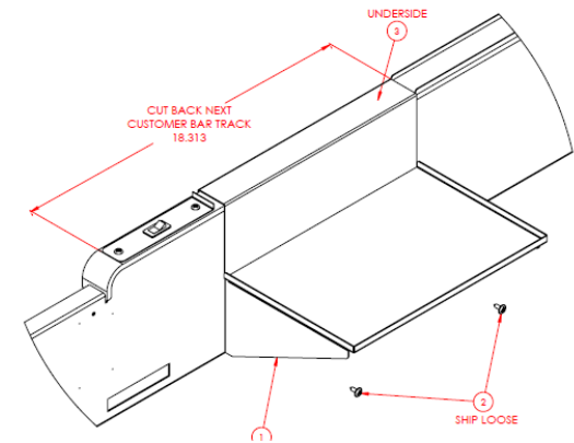
Printer Shelf AS062-100
