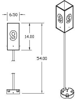
LRO00001 LANE LIGHT RED
