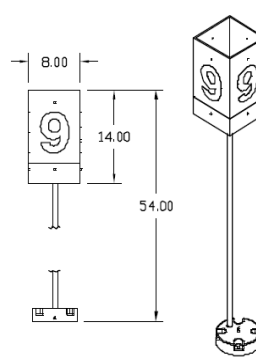
LB000001 LANE LIGHT BLUE W/ STRIPE
